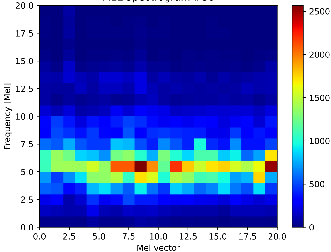
MEL Spectrogram #38
